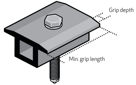
Fig. 1: Clamp specifications
