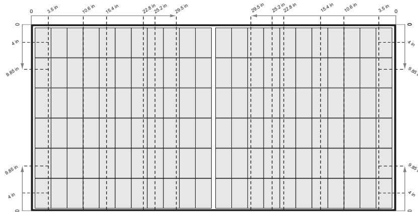
Fig. 11: Clamping of REC Alpha Pure 2 Series panels using short rails
